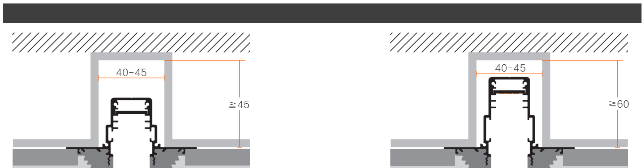
Item No.: KLM-GD7943Y/L1000开孔尺寸: W40*H45mm
